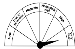
Scheme Benchmark: Solactive Autonomous & Electric Vehicles Index (TRI) (INR)
